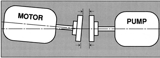
Figure 8.1 Rough angular alignment check using feeler gauges.
