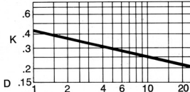
REGULAR FLANGED 90° ELL.
