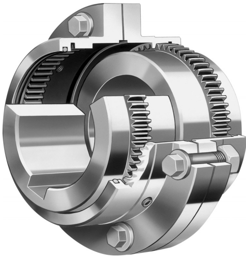
Figure 4.43 Gear coupling. (Courtesy of The Falk Corporation, Milwaukee, WI.)
