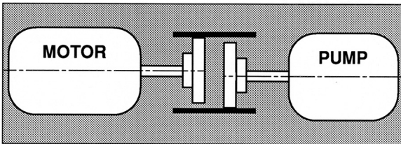
Figure 8.2 Rough parallel alignment check using straight edge.
