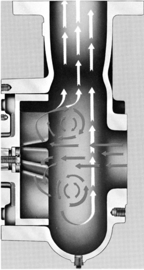
Figure 4.7 Vortex impeller: principle of operation. (Courtesy of Aurora Pumps, North Aurora, IL.)
