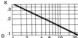
LONG RADIUS FLANGED 90° ELL.
