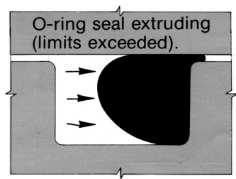
Figure 5.4 O-ring seal with pressure limited exceeded. (Courtesy of Parker Hannifin Corporation, Seal Group.)
